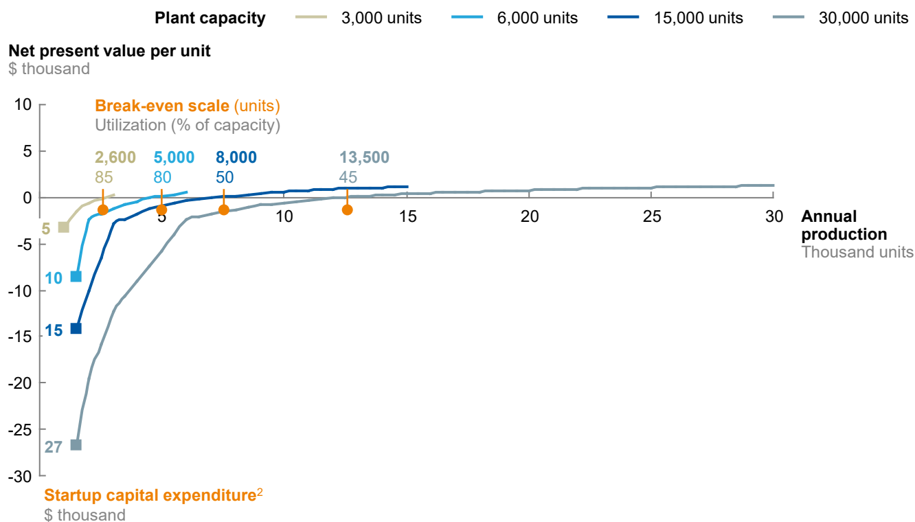
Break-even scale for 3,000- to 30,000-unit pre-cast plants 1
